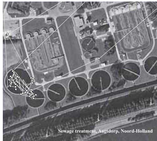
Figure 4. Foraging activity at a sewage treatment near Aagtdorp, Noord-Holland, of a lesser black-backed gull with GPS logger from Kelderhuispolder, Texel. Dots represent individual GPS uploads, white lines represent flights.
